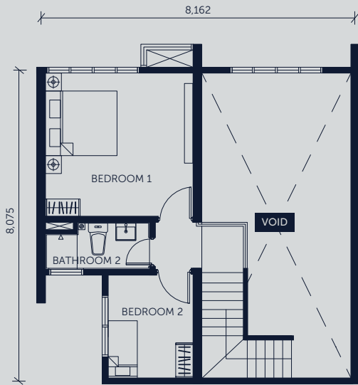
UPPER FLOOR
